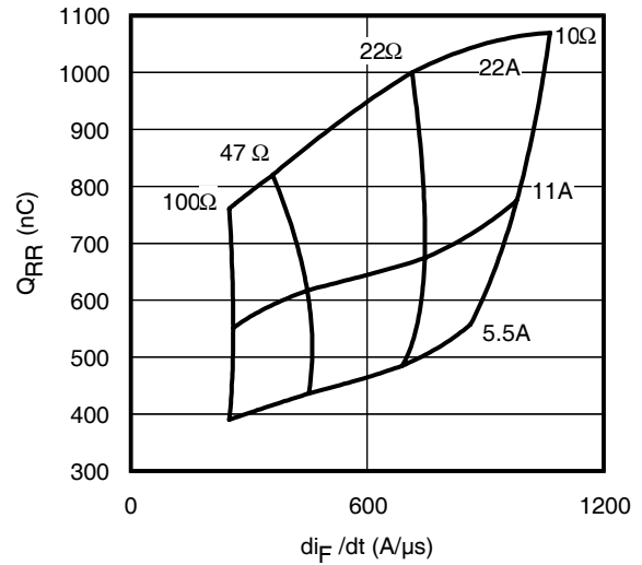
Fig. 20 - Typical Diode Q_{RR} V_{CC}= 400V ; V_{GE}= 15V ; T_J = 150^{\circ}C
